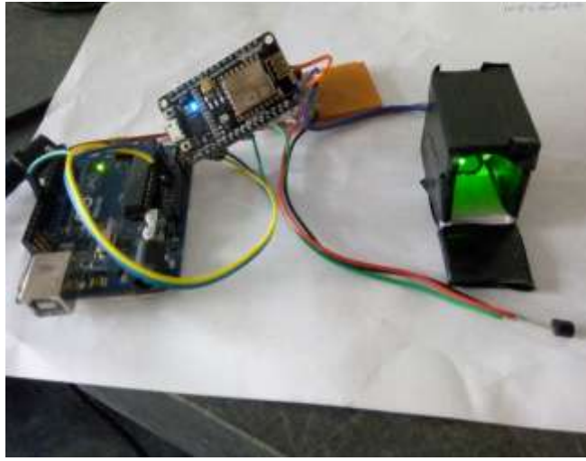
Fig no. 5 vein detection system
