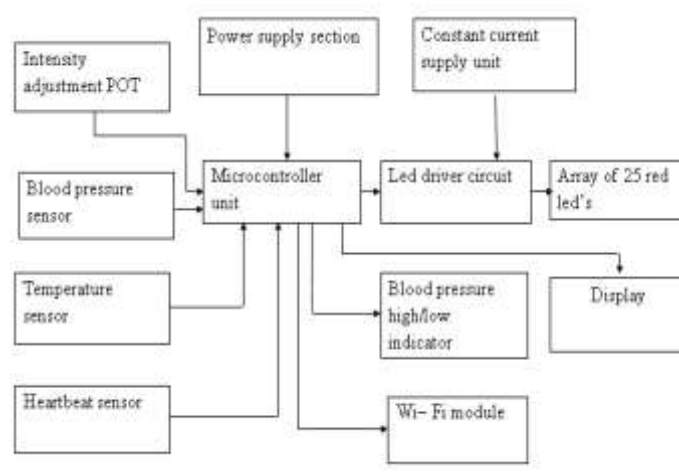
Fig no. 3 Block diagram of the system
