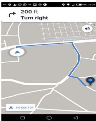
Fig. 7. Navigation Activity
