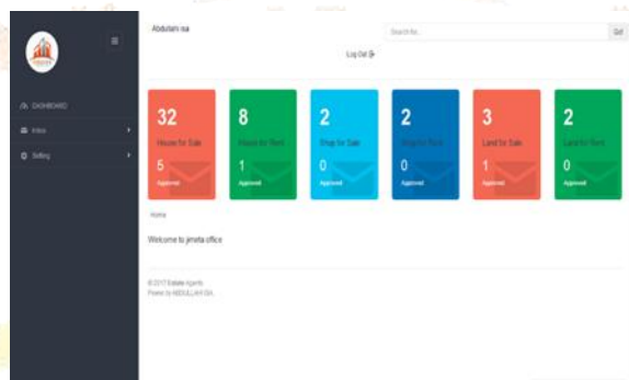
Fig. 8. Agent Dashboard
