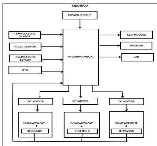
Fig 1: block diagram of Medibox
