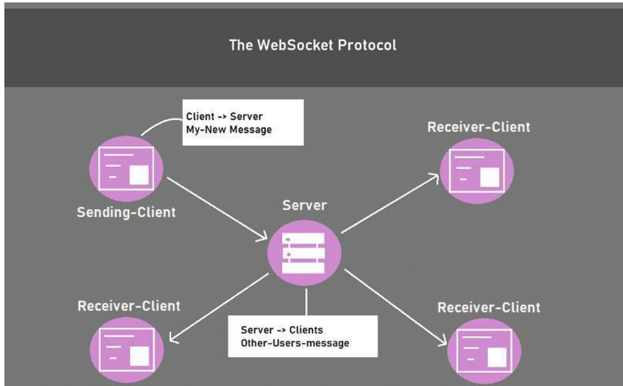
Figure 5: WebSocket Protocol: Event of Sending a message
