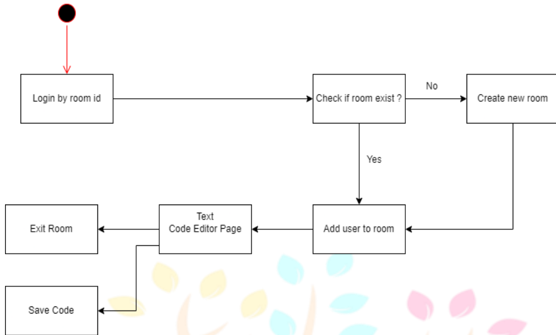
Figure 1: UML Diagram of Realtime Code Editor
