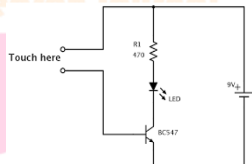
Fig 4.9 Circuit diagram of touch sensor
