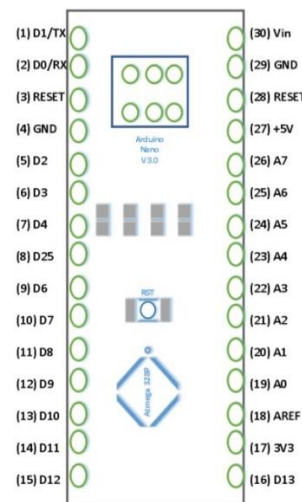
Fig 4.2 Arduino Nano Pin out
