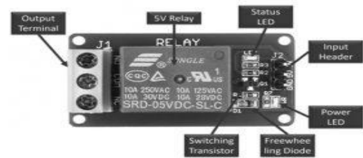
Fig 4.6 5V 1-Channel relay module components
