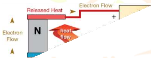
Heat Transfer In "N" type
