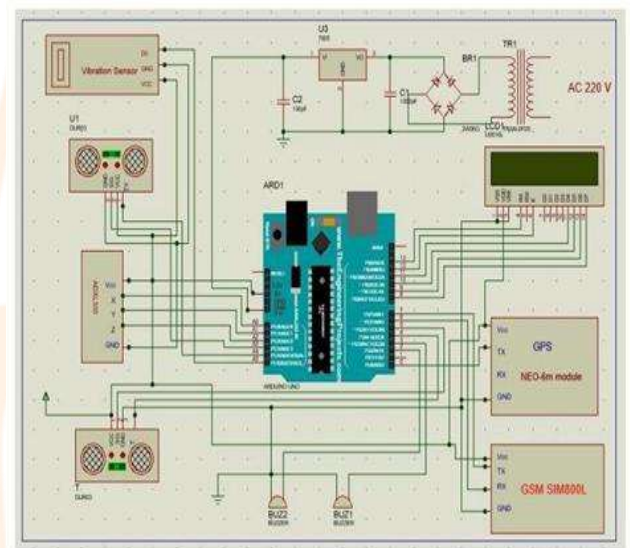
Fig 1.6 Circuit Diagram
