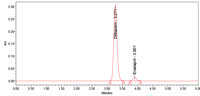
Figure 10: Chromatogram for Linearity 4
