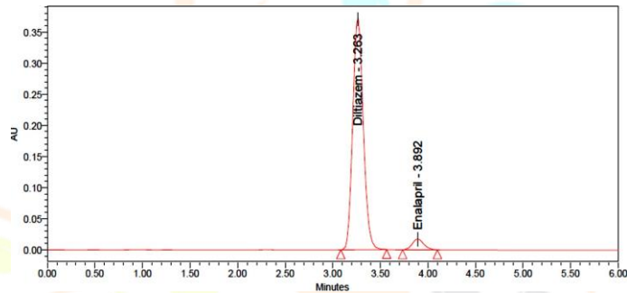
Figure 11: Chromatogram for Linearity 5
