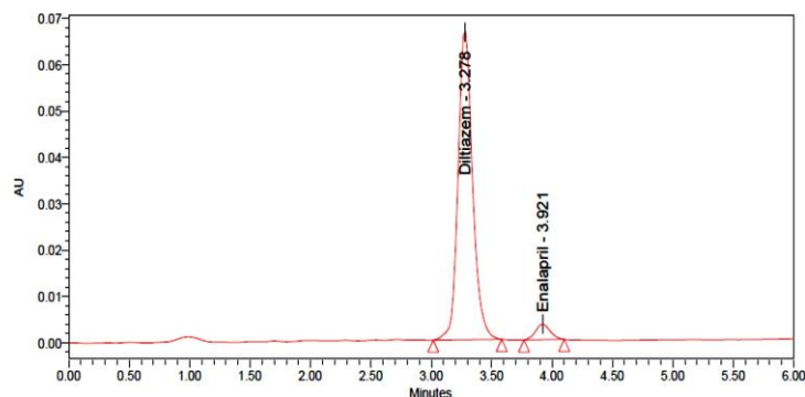
Figure7: Chromatogram for Linearity 1
