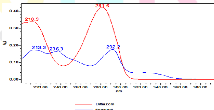
Fig. 3: Overlaid Spectrum of Diltiazem HCl & Enalapril Maleate
