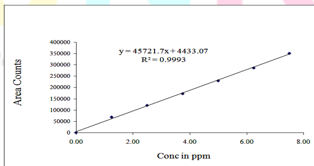
Figure 6: Calibration curve for Enalapril Maleate at 236nm
