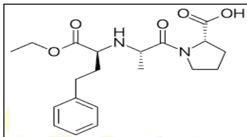
Fig. 1. Structure of Enalapril Maleate
