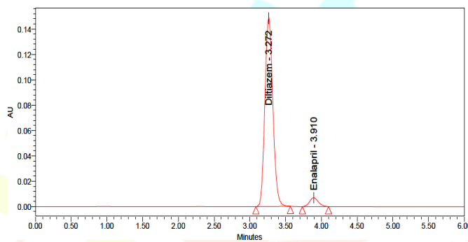
Figure 8: Chromatogram for Linearity 2
