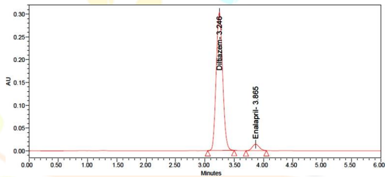
Figure 6. Chromatogram of Sample Solution
