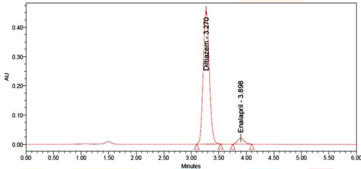
Figure 12: Chromatogram for Linearity 6
