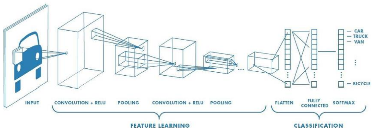
Fig. 6 CNN ARCHITECTURE [14]
