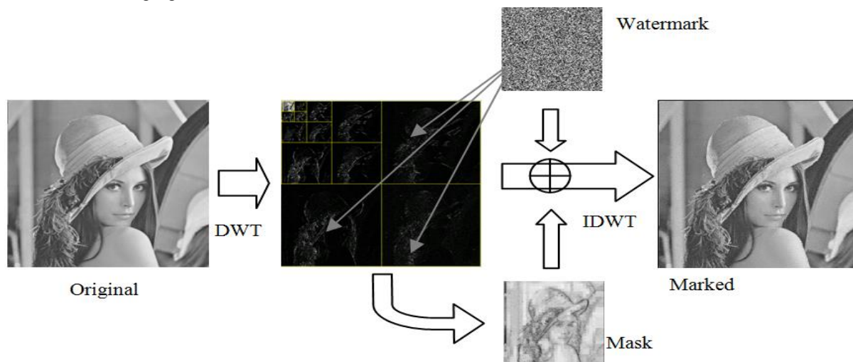
Figure 2. Watermark embedding in the wavelet domain (Barni et al., 2001). The watermark is embedded in the first resolution level using a perceptual mask.
