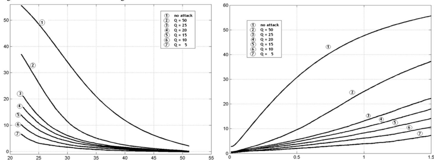
Figure 6. Left: The ratio \rho/T as a function of the PSNR between the marked and the original images, for different quality factors, JPEG compression. Right: Ratio \rho/T as a function of embedding strength, for different quality factors, JPEG compression. P_f is set to 10^{-8} .
