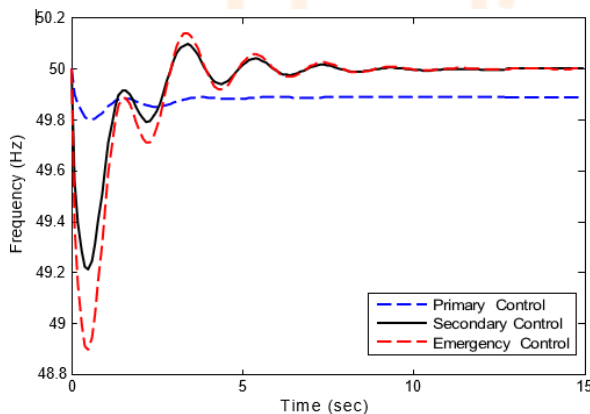
Fig. 4 Primary, secondary and emergency control
