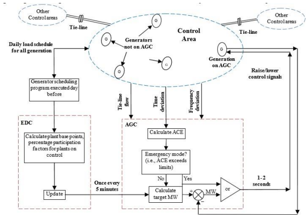
Fig. 5 Functional diagram of typical AGC system
