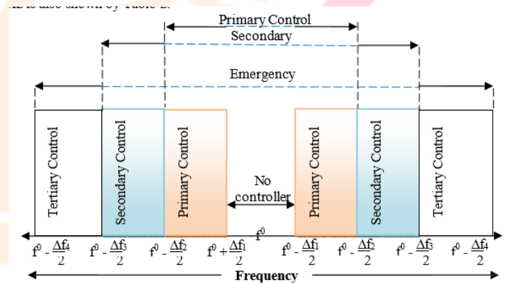
Fig. 2. Frequency deviations and associated operating controls
