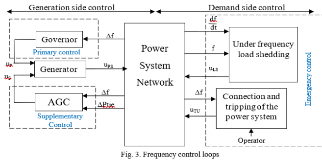
Fig. 3. Frequency control loops
