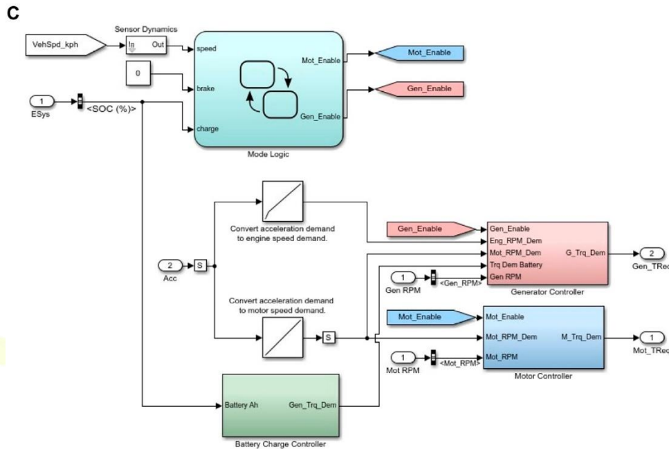
FIGURE 8 | Simulink Models of (A) Block of a BEV (Chen and Rincon-Mora, 2006) (B) Electrical system configuration and (C) Control system configuration.
