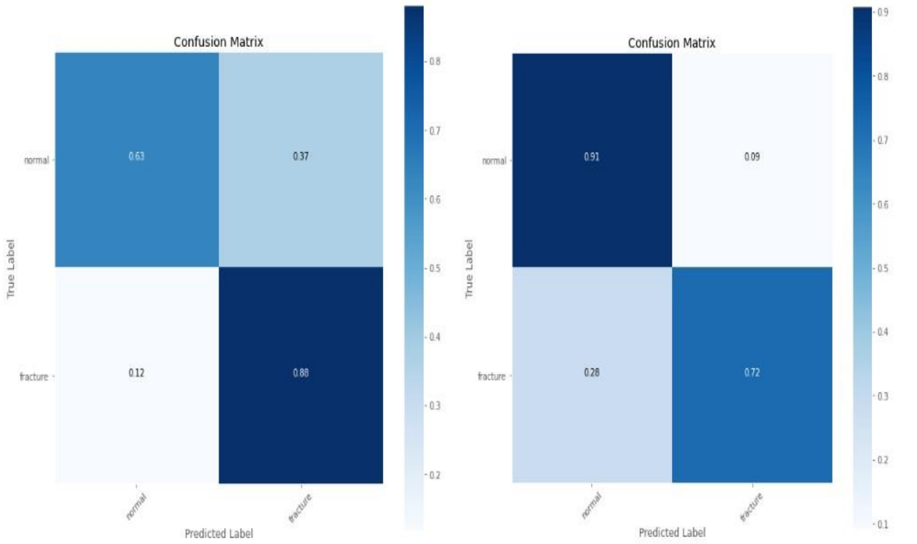
R-CNN Confusion Matrix for validation dataset results Predicted accuracy fracture: 88% and normal: 63%
