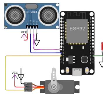
Fig 4: Slave Device Esp32 Circuit diagram (Example IOT Device)
