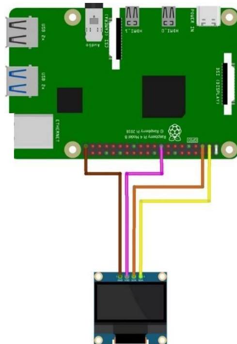
Fig 3: Master Device (Rpi) Circuit diagram
