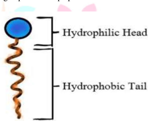
Figure 1: Single Amphiphilic Molecule
