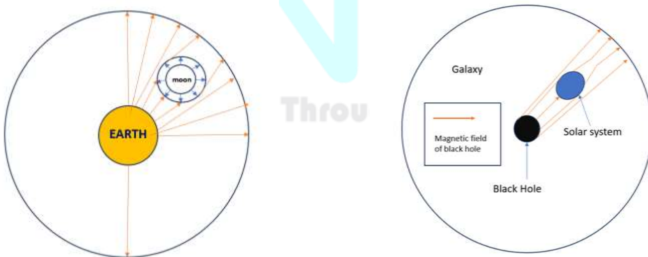
Fig 6. This image shows how the gravitational force of Earth is applied to the Moon and how the gravitational force of the black hole applied on solar system.
