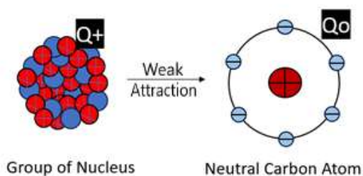
Fig 3. This figure showing the interaction of a group of nuclei with a neutral atom.
