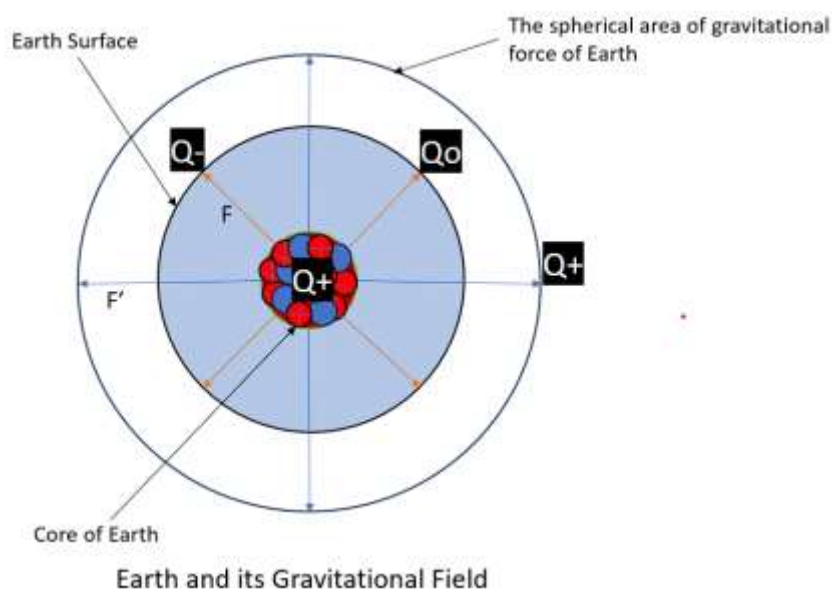
Fig 4. Showing that location of nuclei presents in core of earth, and how gravitational force of earth work.
