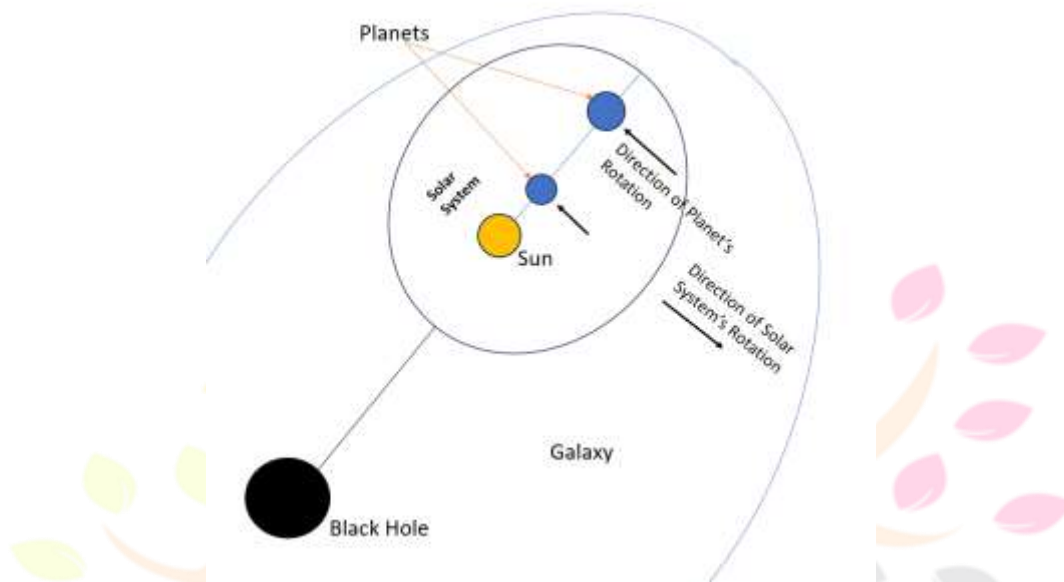
Fig 7. This image shows the rotation of the planets and the solar system around the black hole in the galaxy.
