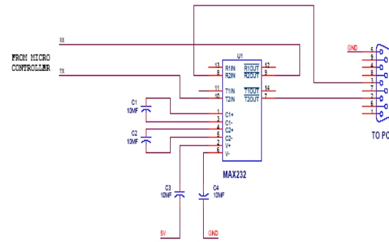
Figure 3 MAX 232 Circuit
