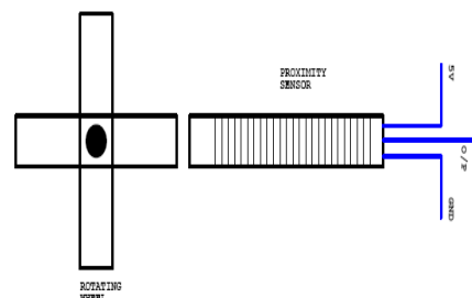
Figure 4 Proximity Sensor
