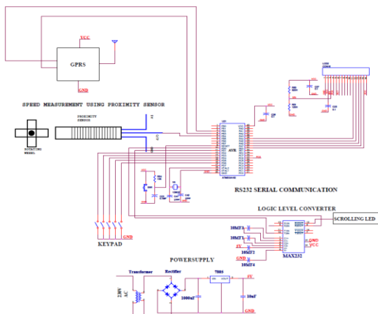
Figure 5 Circuit Diagram of the Hardware implementation
