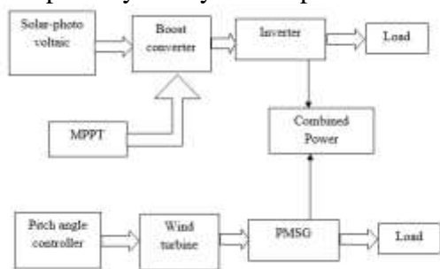
Fig 1. Block diagram of hybrid system
