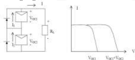
Fig 2. Series connection of PV cells
