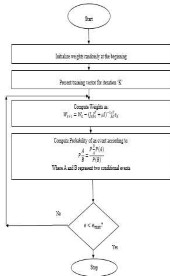
Fig.3 Flowchart for training
